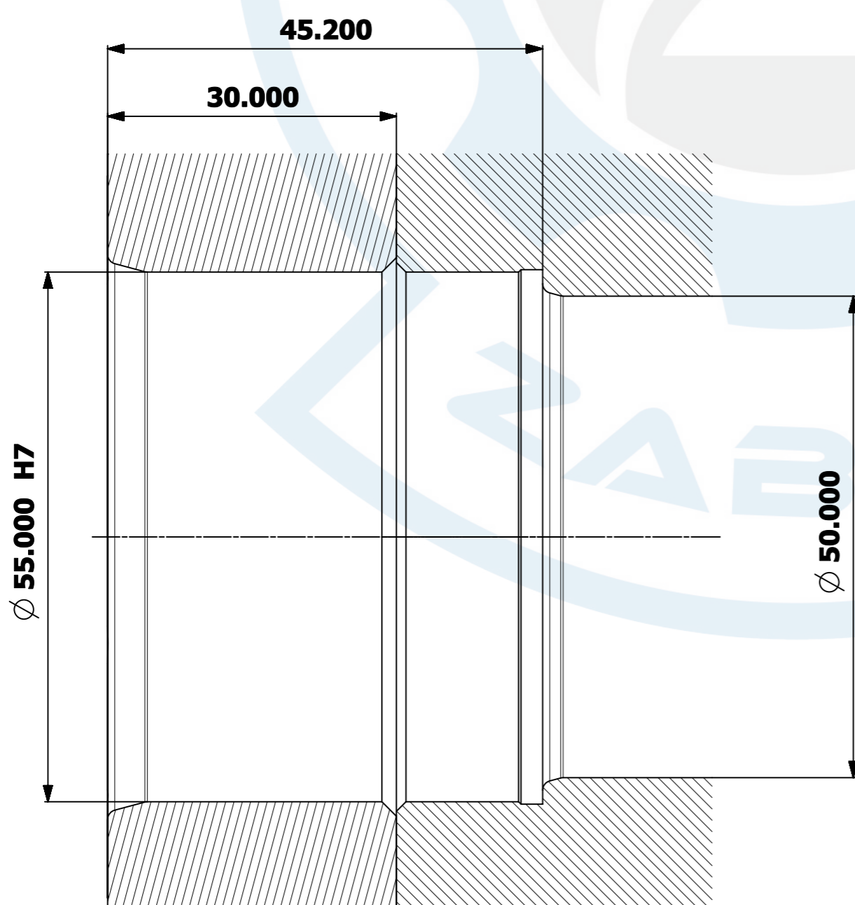
CENTER BORE DETAIL
