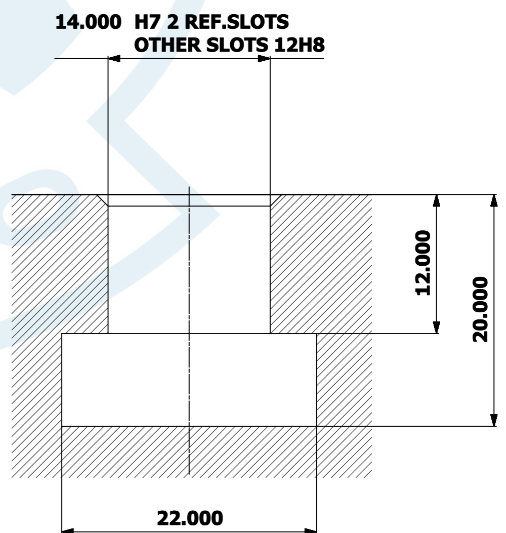
T-SLOTS DETAILS
